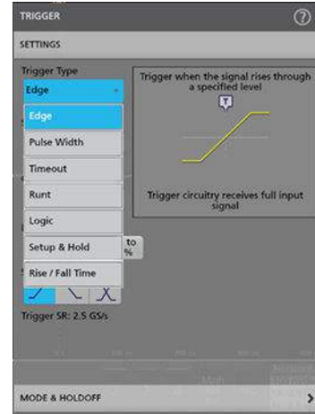
Configuration menus are accessed by simply double tapping on the item of interest. In this case trigger badge was tapped to open trigger menu.
